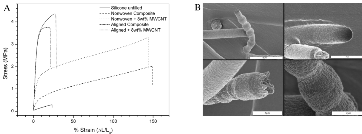
Figure 1: Stress-strain curves (A) for the various silicone composites and SEM images (B) of the composite fracture surface showing fibre pullout and yielding.
